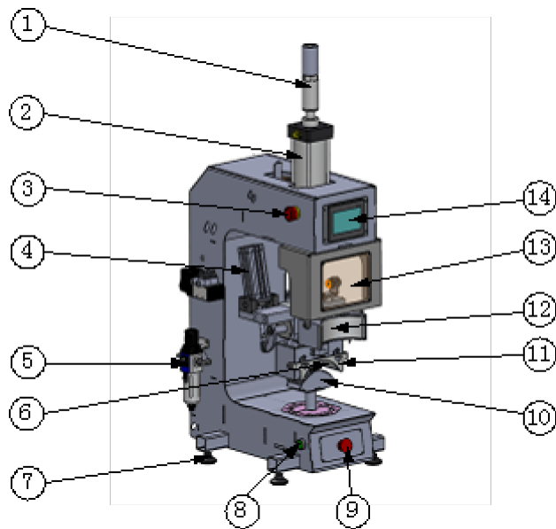
Fig.2 Machine parts name
